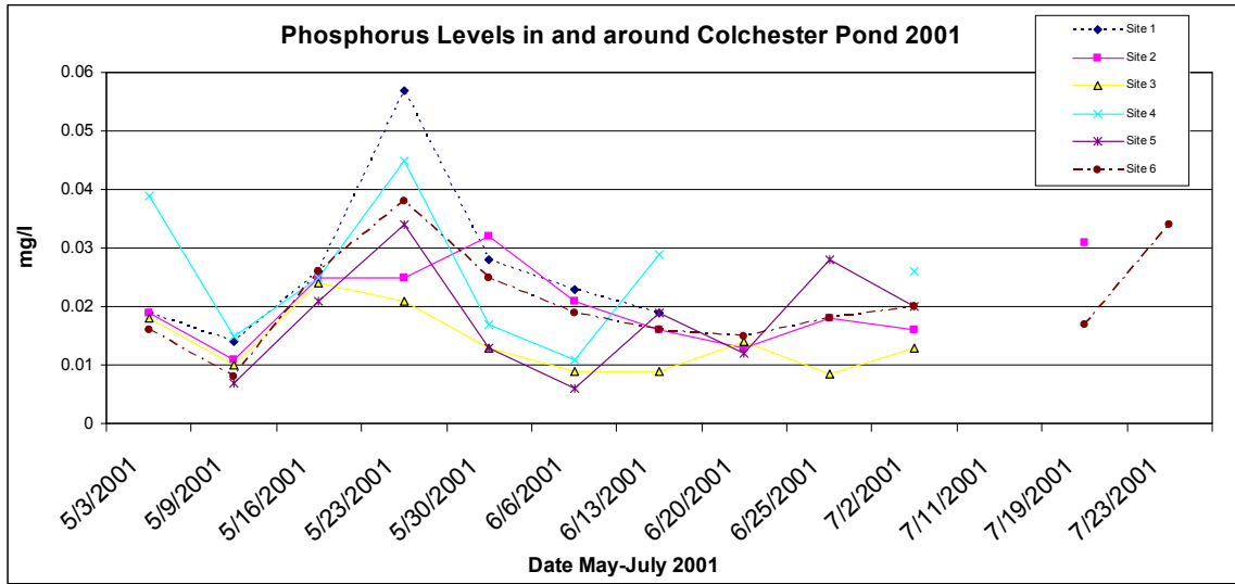
Fig. 7. Phosphorous levels in and around Colchester Pond 2001
