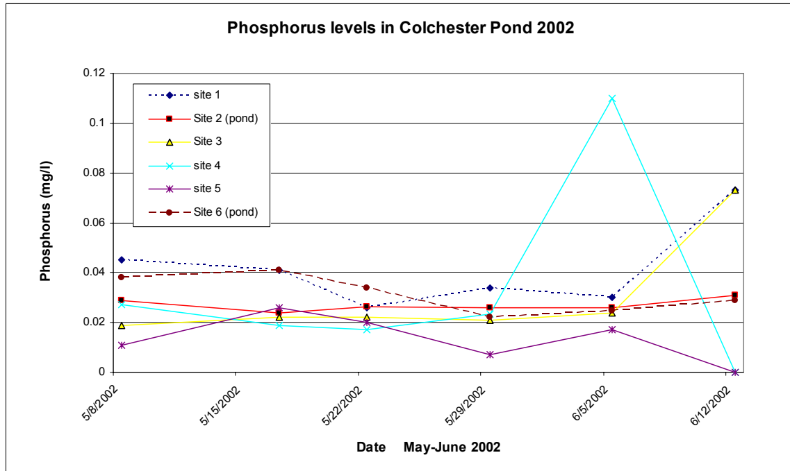
Fig. 8. Phosphorous levels in Colchester Pond 2002
