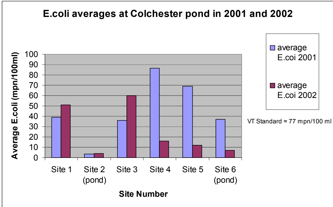
Fig. 3. E. coli averages at Colchester Pond in 2001 and 2002
