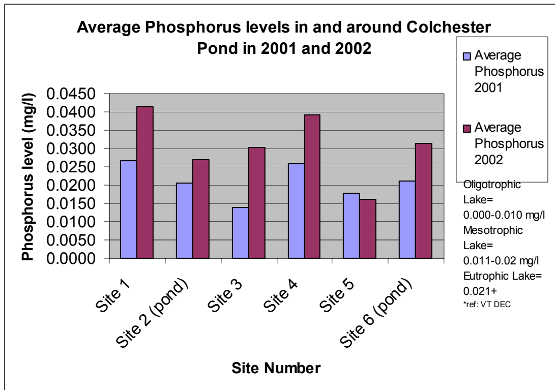
Fig. 6. Average Phosphorus levels in and around Colchester Pond in 2001 and 2002
