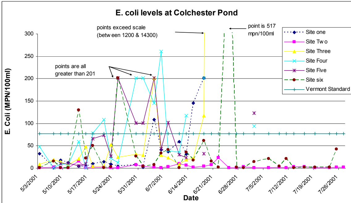
Fig. 4. E. coli levels at Colchester Pond 2001
